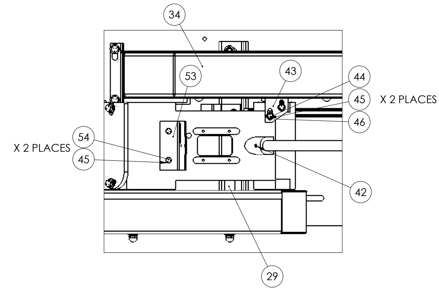
TOP VIEW OF ARM, GUARDS, SPACER #28 DETAIL, SET SCREW FOR HANDLE, AND FASTENERS FOR INTERNAL WHEEL GUARD
