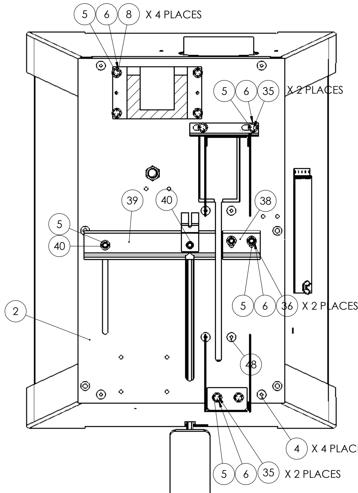
SECTION A-A MOUNTING TO BASE PLATE
